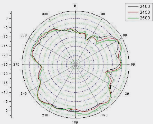
2.4G (PHI=0)
