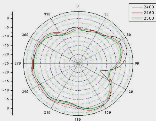
2.4G (PHI=90)
